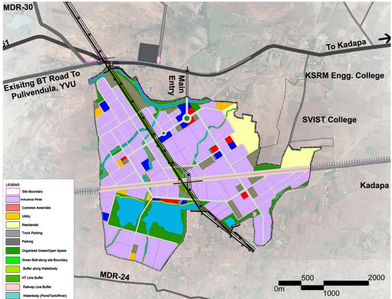
Figure 3: Master Plan of Kopparth Industrial Area
